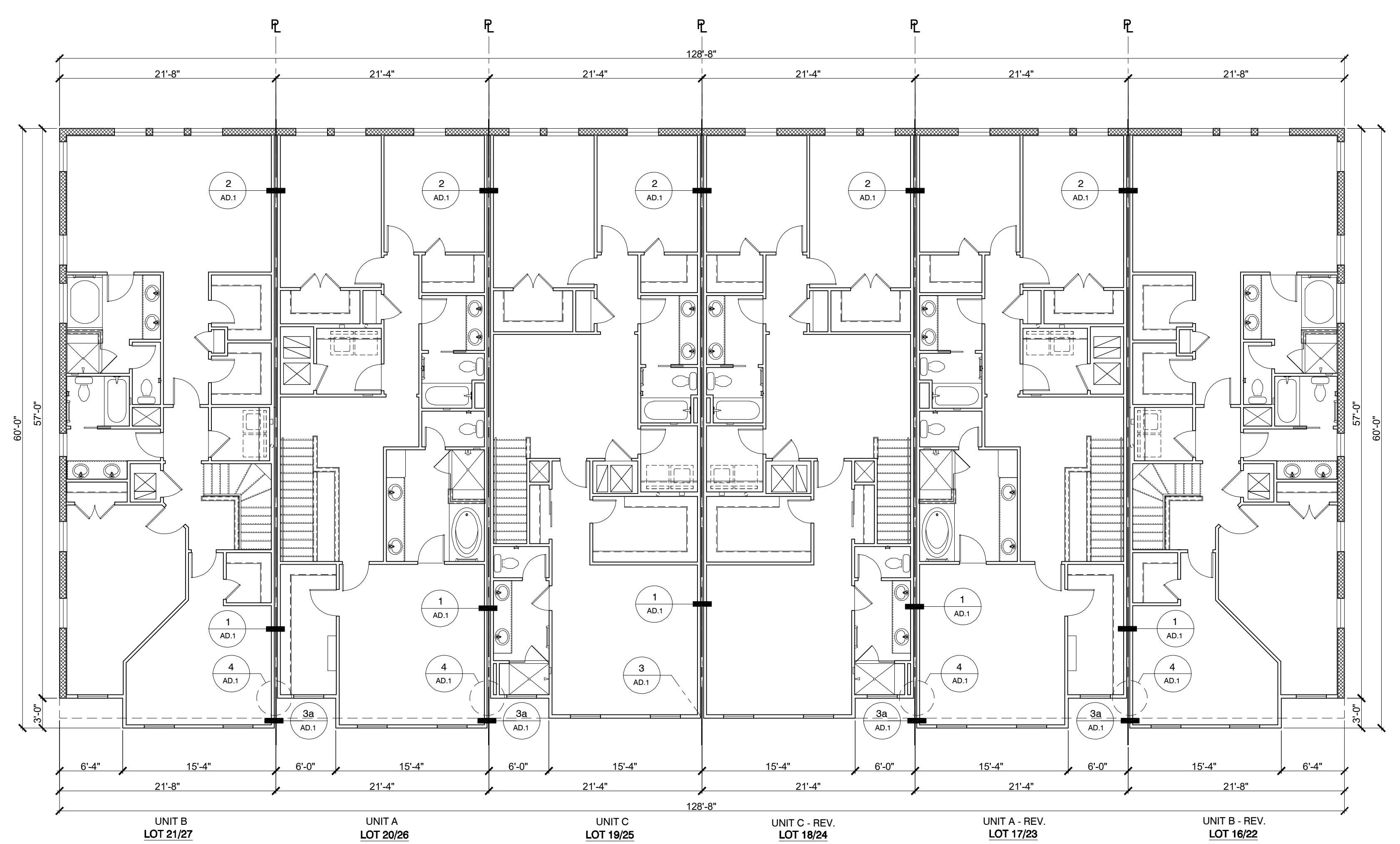
6 UNIT BUILDING - SECOND FLOOR
