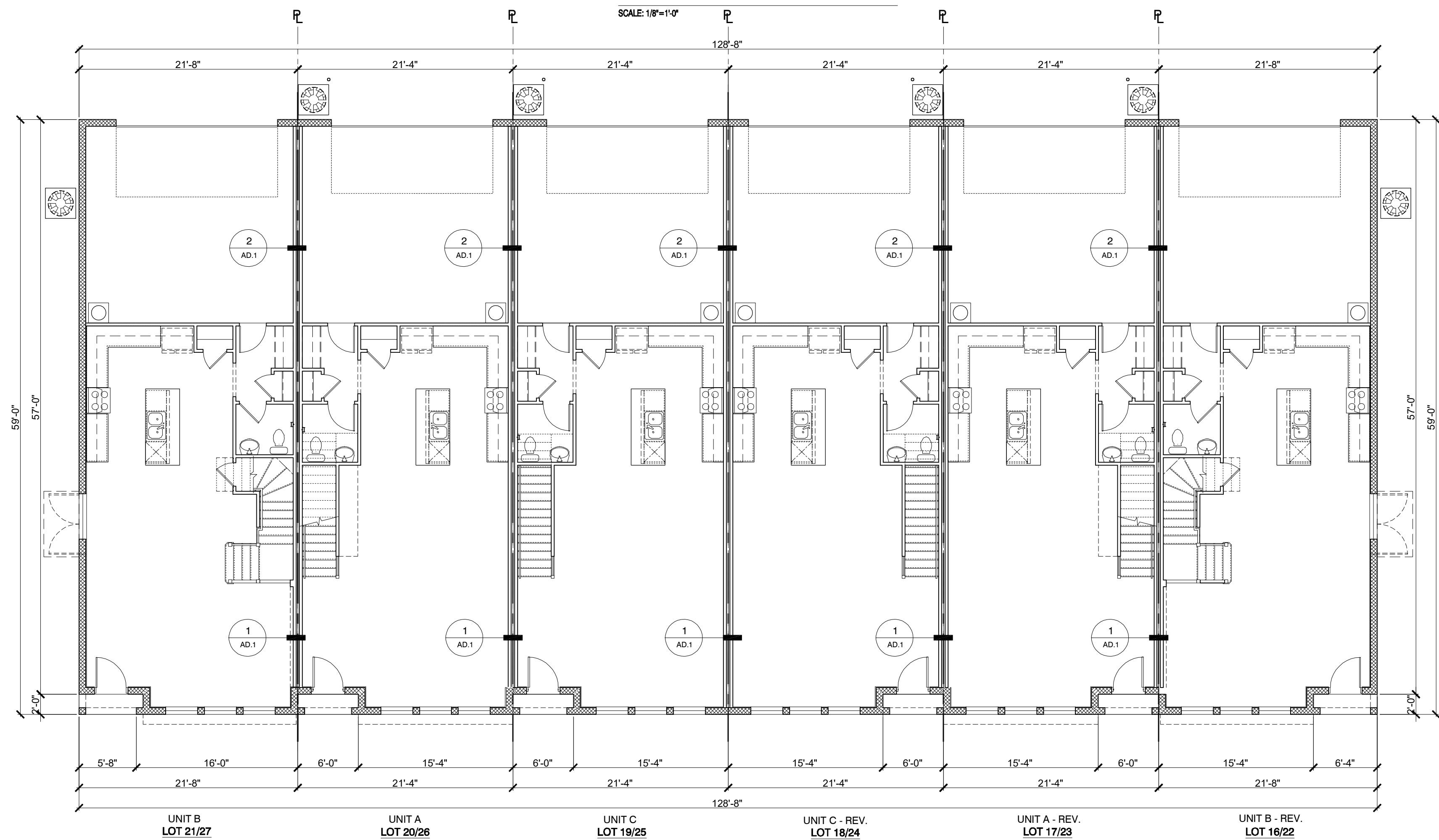
6 UNIT BUILDING - FIRST FLOOR
